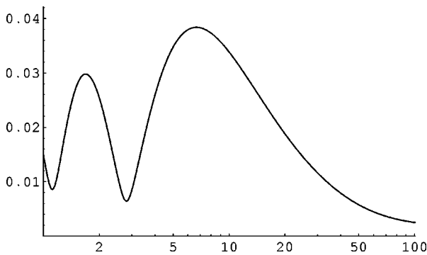
FIG. 2. The \beta dependence of the spectrum, P_k^{1/2} , is plotted against \beta , with H=0.1 . For a de Sitter background, the spectrum is independent of k .
