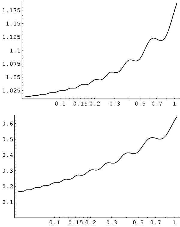
FIG. 3. The values of D_+ (top) and D_- are extracted for the spectrum shown in Fig. 1 with C_- = 0 . As \beta \rightarrow 0 , D_+ \rightarrow 1 and D_- \rightarrow 0 , confirming that as the Hubble length becomes much larger than the minimum length the spectrum approaches the standard result.
