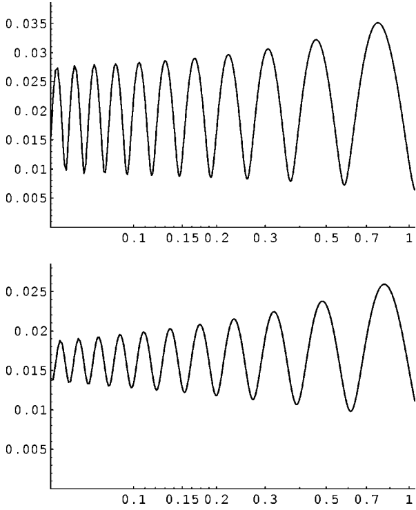
FIG. 1. The top figure shows the spectrum ( P^{1/2} ) as a function of \beta with C_-/C_+ = -0.5 , while the lower plot shows the spectrum when C_- = 0 . It is only in the latter case that the computed value of the spectrum smoothly approaches the usual value in de Sitter space. In this plot H=0.1 , and with \beta=0 we would expect P^{1/2} = 0.0159155 .
